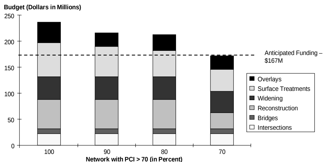
Figure 6.5 KCRC Future Pavement Condition
